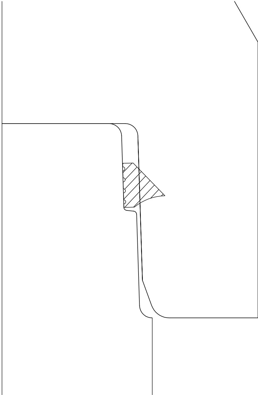
RUBBER GASKET ASTM C-443 JOINT
